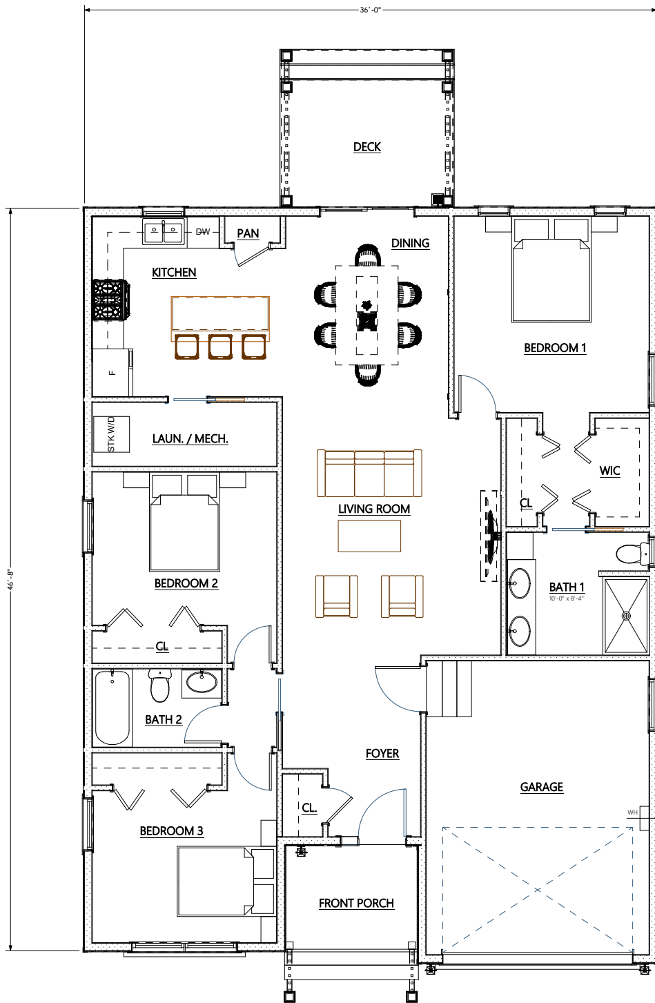
LOT 2 - FLOOR PLAN
